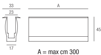
Cassaforma con bordo Anodized aluminium profile
