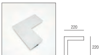
Curva piana 90° senza Led 90° plane corner without Led
