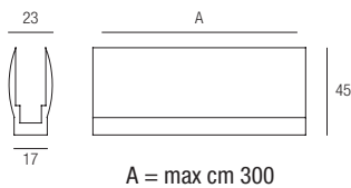
Cassaforma senza bordo Anodized aluminium profile
